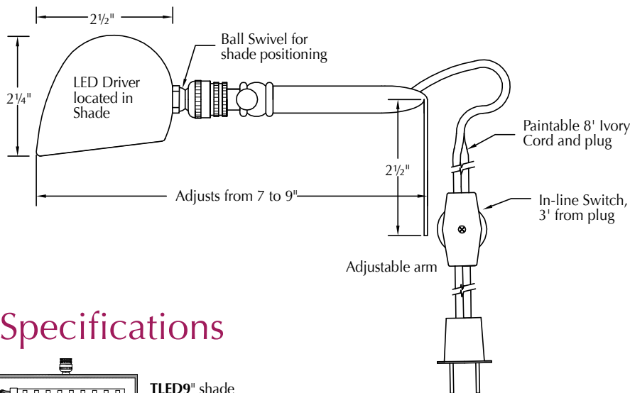
TLED9" shade 2.4 Watt, 100 Lumen LED
