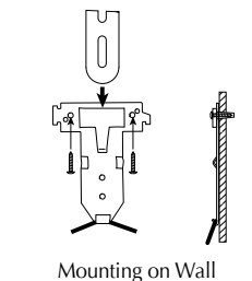
Mounting on Wall
