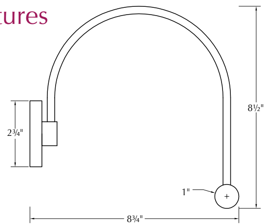
DXL36" shade six 15T4 bulbs included BACKPLATE: 2 3/4" x 17 1/2"
