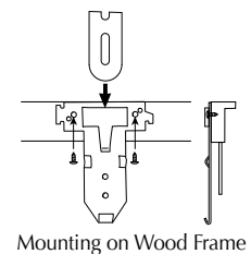
Mounting on Wood Frame
