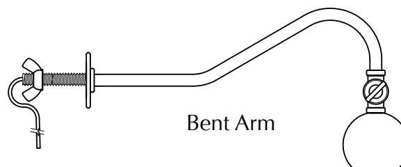
Hyde Park Shade (Refer to page 153 for shade width and finish options.)
